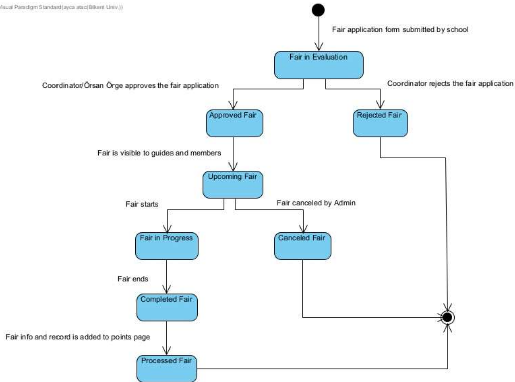
Figure 13: The state diagram of a fair object
