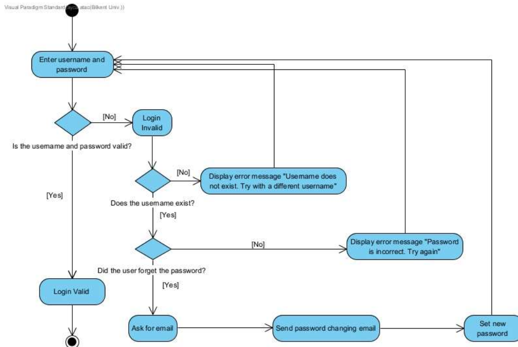
Figure 2: The login operations for members with accounts
