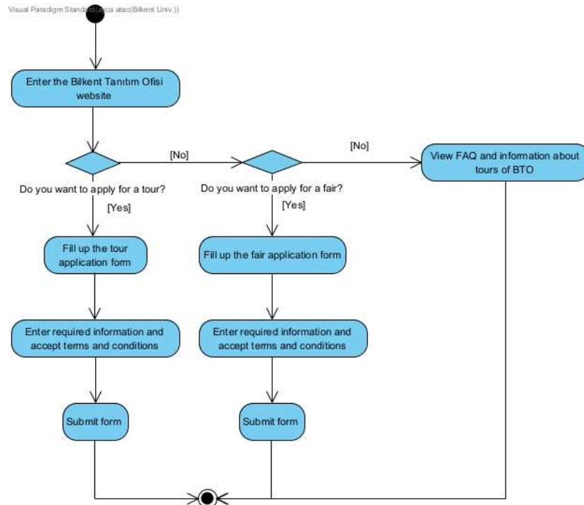
Figure 1: The viewing and applications of the BTO website for users without accounts
