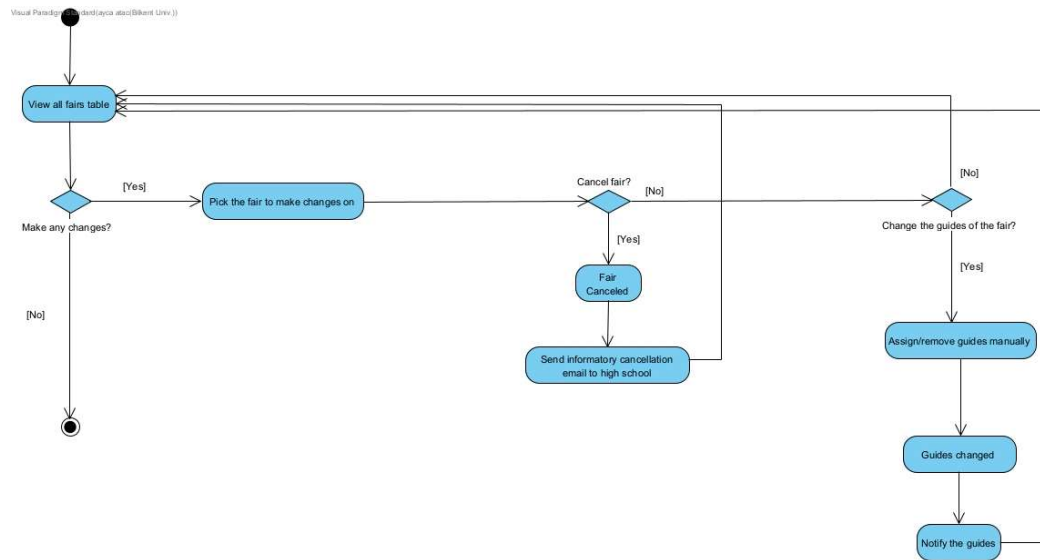
Figure 7: The cancelation and editing of already existing and approved fairs by the coordinator or director
