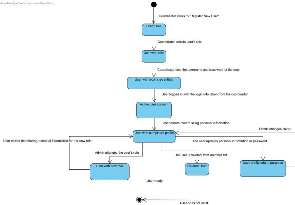
Figure 14: The state diagram of a user object
