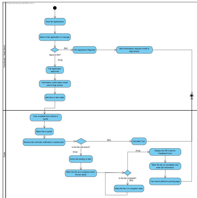
Figure 6: The management of fairs from application to completion.
