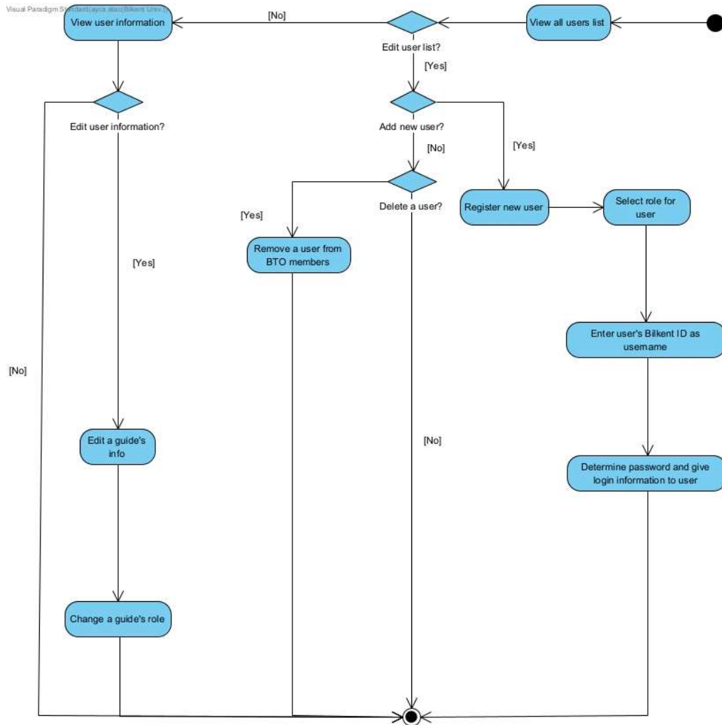
Figure 8: The management (adding a user, deleting a user, changing the role of a user) of the members list
