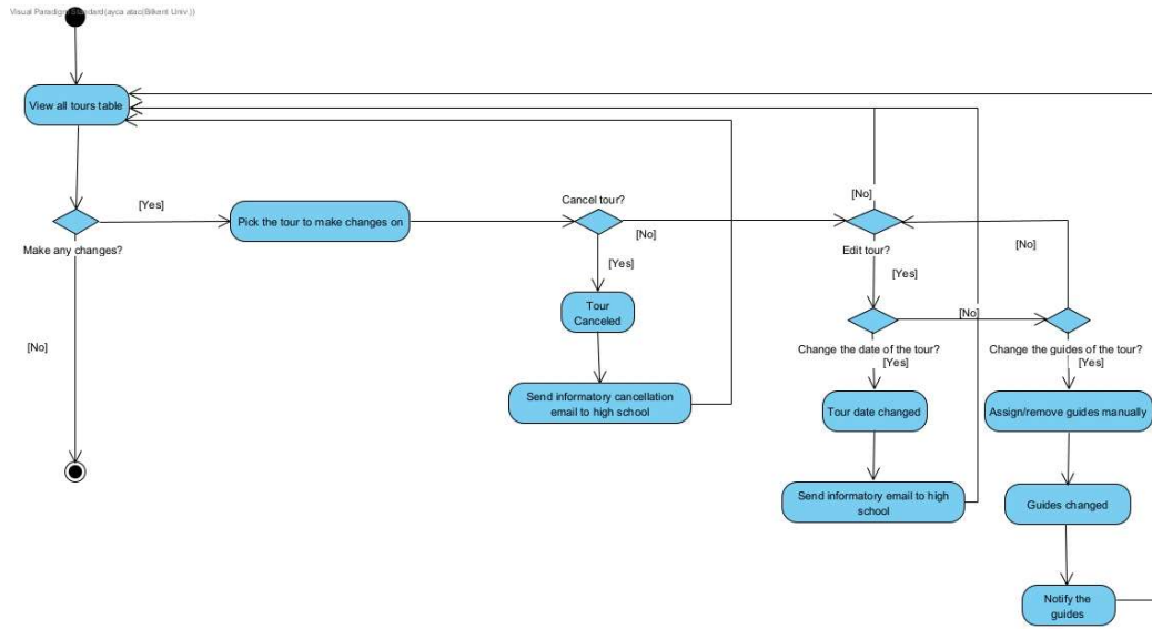
Figure 5: The cancelation and editing of already existing and approved tours by the head secretary
