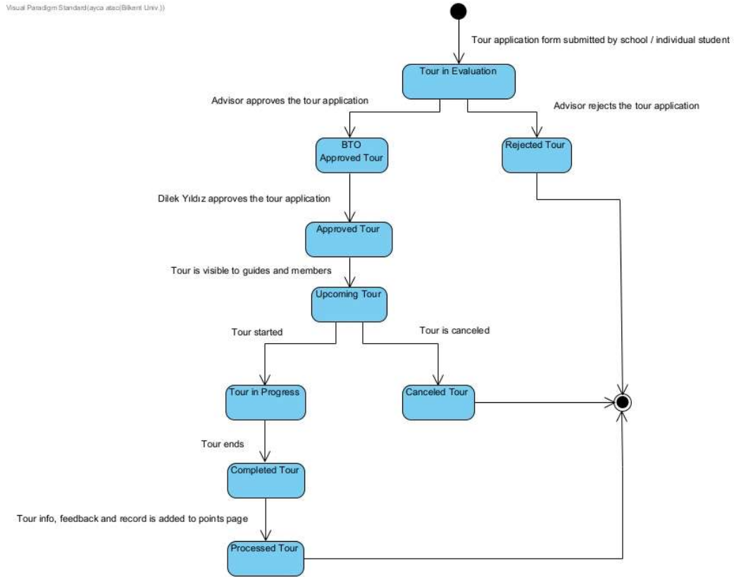
Figure 12: The state diagram of the tour object
