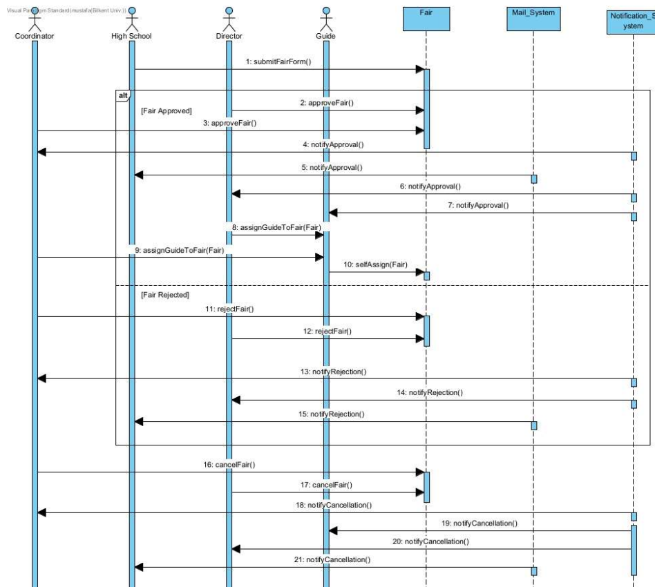
Figure 10: Fair Management Sequence Diagram
