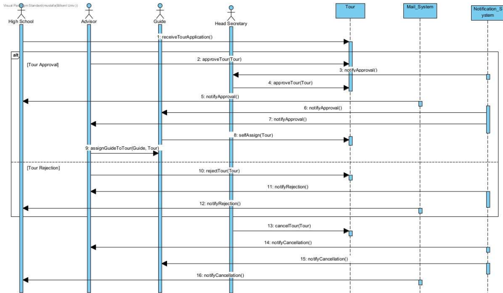
Figure 9: Tour Management Sequence Diagram
