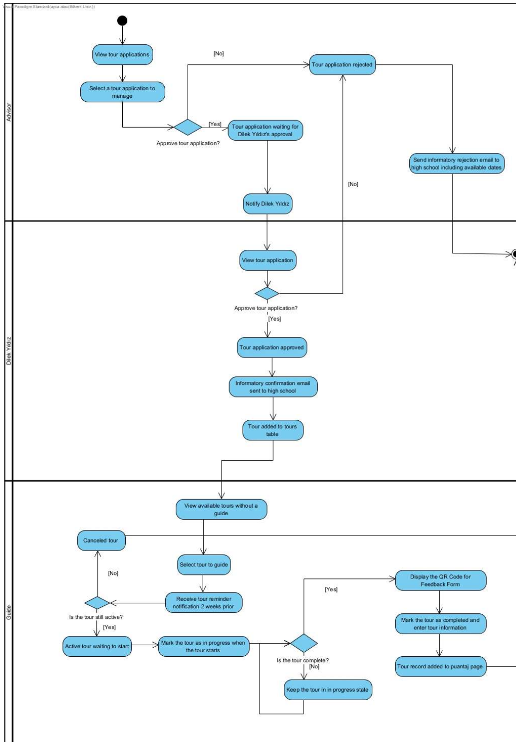
Figure 4: The management of tours from application to completion.
